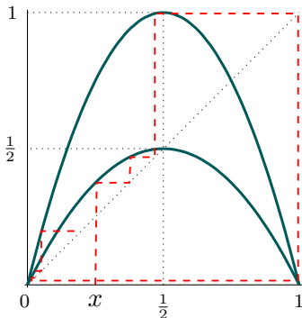
FIGURE 1. Critical intermittency in the random system of logistic maps T_2 , T_4 . The dashed line indicates part of a random orbit of x
