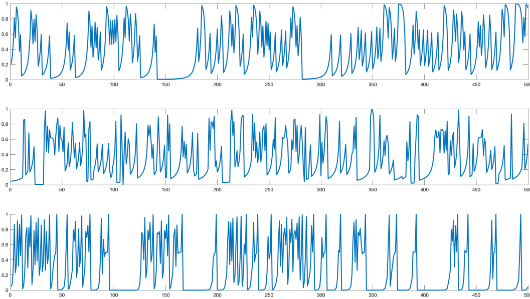
FIGURE 2. Intermittent behaviour of orbits of (a) a single Manneville-Pomeau map with \alpha = 1.5 , (b) a random mixture of the Gauss and Rényi continued fractions maps where the Gauss map is chosen with probability p = 0.1 and (c) a random mixture of the logistic maps T_2 and T_4 where the map T_4 is chosen with probability p = 0.6 .
