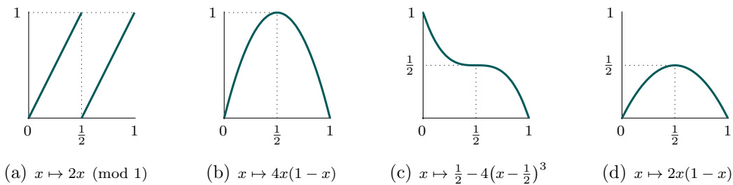
FIGURE 3. Four maps with critical point c = \frac{1}{2} . (a) and (b) show two good maps, while in (c) and (d) we see the graphs of two bad maps.
