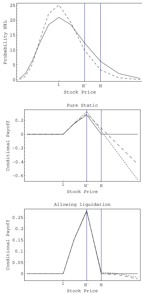
Figure 6: Hedging consistently with a pricing functional using the risk-neutral probability distribution and another probability distribution. The upper panel shows the risk-neutral, lognormal, probability distribution (dashed line) and the one based on the equiprobability of paths (solid line). The conditional portfolio payoffs following pure static strategies are displayed in the middle panel; those based on strategies allowing liquidation in the lower panel. In both cases, the long-dashed curves represent the conditional payoffs when mean-square hedging uses the risk-neutral (lognormal) probability distribution; the short-dashed curves show the conditional payoffs when hedging is based on the equiprobability of paths; H^- denotes the barrier and H^- the highest possible stock price lower than the barrier. H^- is the strike of a regular option used in hedging; H is not.
