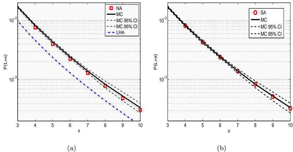
Figure 3: The loss distribution obtained from (a) the large homogeneous approximation (LHA), the normal approximation (NA) and (b) the saddlepoint approximation (SA) compared to results based on Monte Carlo (MC) simulation of two hundred thousand scenarios. The MC 95% confidence interval (CI) are based on the standard deviation calculated using 10 simulated sub-samples of 20 thousand scenarios each.
