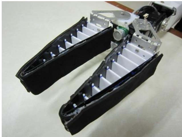
Fig. 5. An ultrasonic sensor for detecting grasped objects
