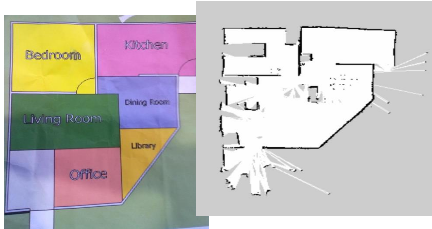
Fig. 10. Mapping of the house created by data from a 2D laser range-finder
