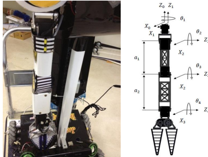
Fig. 3. The 4-DOF robot arm with a fin-ray effect gripper [2]
