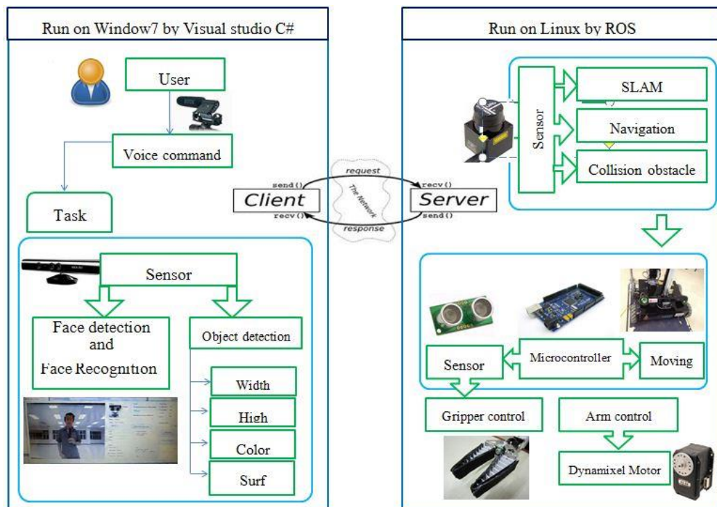
Fig. 9. The diagram of the robot control system
