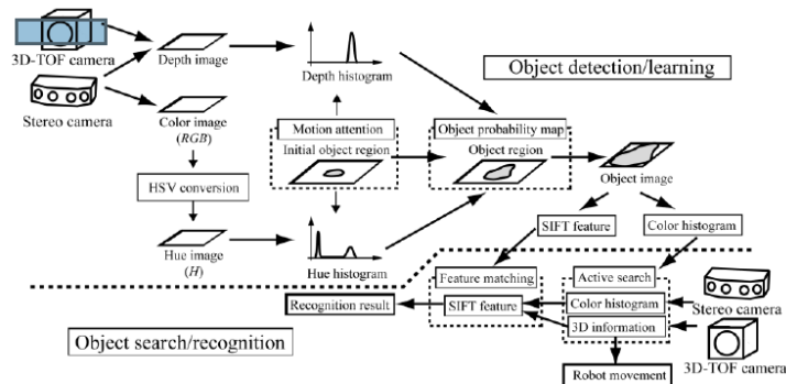
Fig. 2. Processing in the vision module
