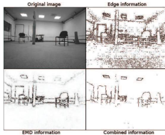
Figure 3: Example [Gerke et al., 2011] of EMD for the removal of spurious edges.
