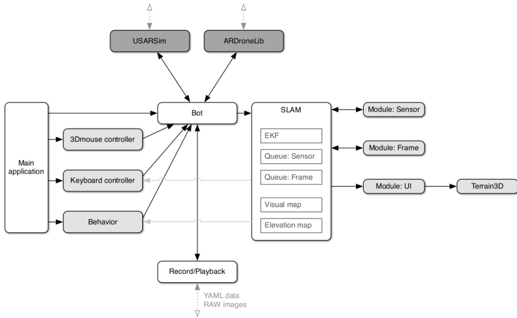
Figure 16: Schematic overview [Dijkshoorn, 2012] of the development framework AR.Drone SLAM
