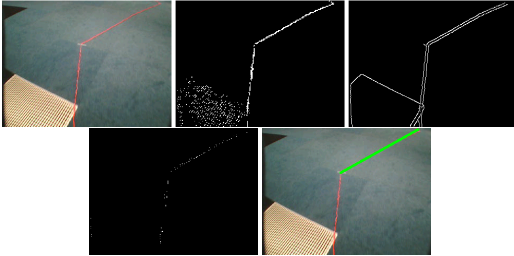
Figure 11: First row: Original Image, Colour Filter and Canny Edge Detector. Second row: Combined Image and the Probabilistic Hough Transform result.
