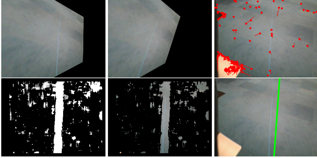
Figure 12: First row: Left Image, Right Image and Optical Flow. Second row: Disparity Map, Disparity Map on Image and the Probabilistic Hough Transform result.
