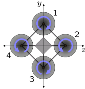
Figure 14: Diagram of the reaction torques on each motor of the quadcopter, due to the rotors. Rotors one and three are spinning clockwise, whereas rotor two and four spin counter-clockwise, causing opposing force for control
