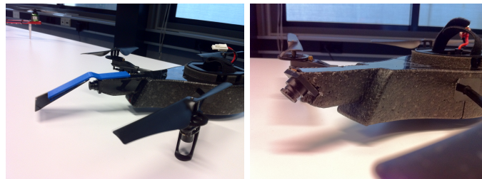
Figure 9: Possible solutions to solve the camera configuration problem, the mirror construction (left) and the modification of the AR.Drone (right)
