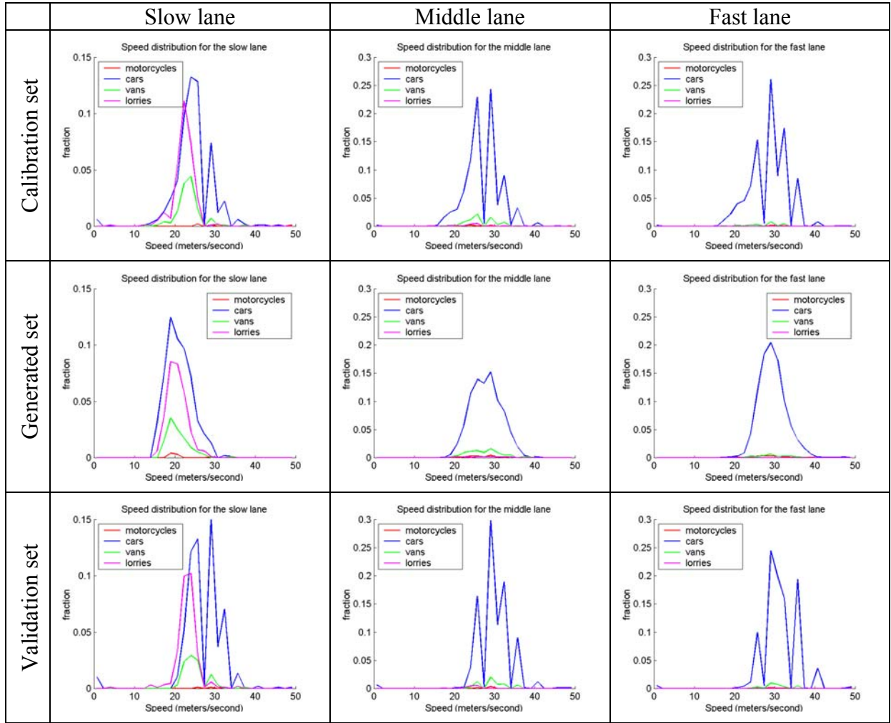
Figure 7: The speed distributions, both measurements and generated.
