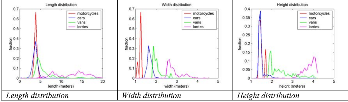
Figure 4: Distribution of the dimensions of the 4 vehicle types.
