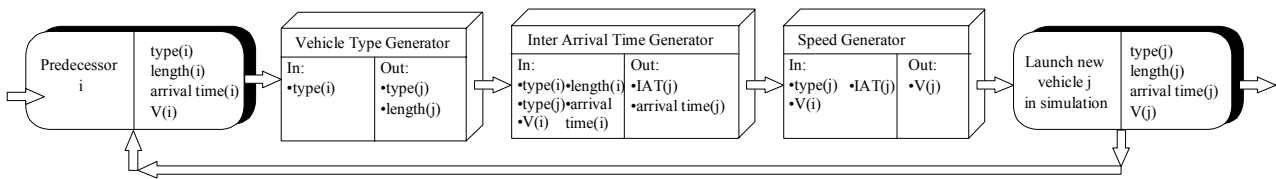
Figure 2: Basic structure of the Random Traffic Generator for Free Flowing traffic. The newly generated vehicle is indicated by the index j ; its predecessor is indicated by i .
