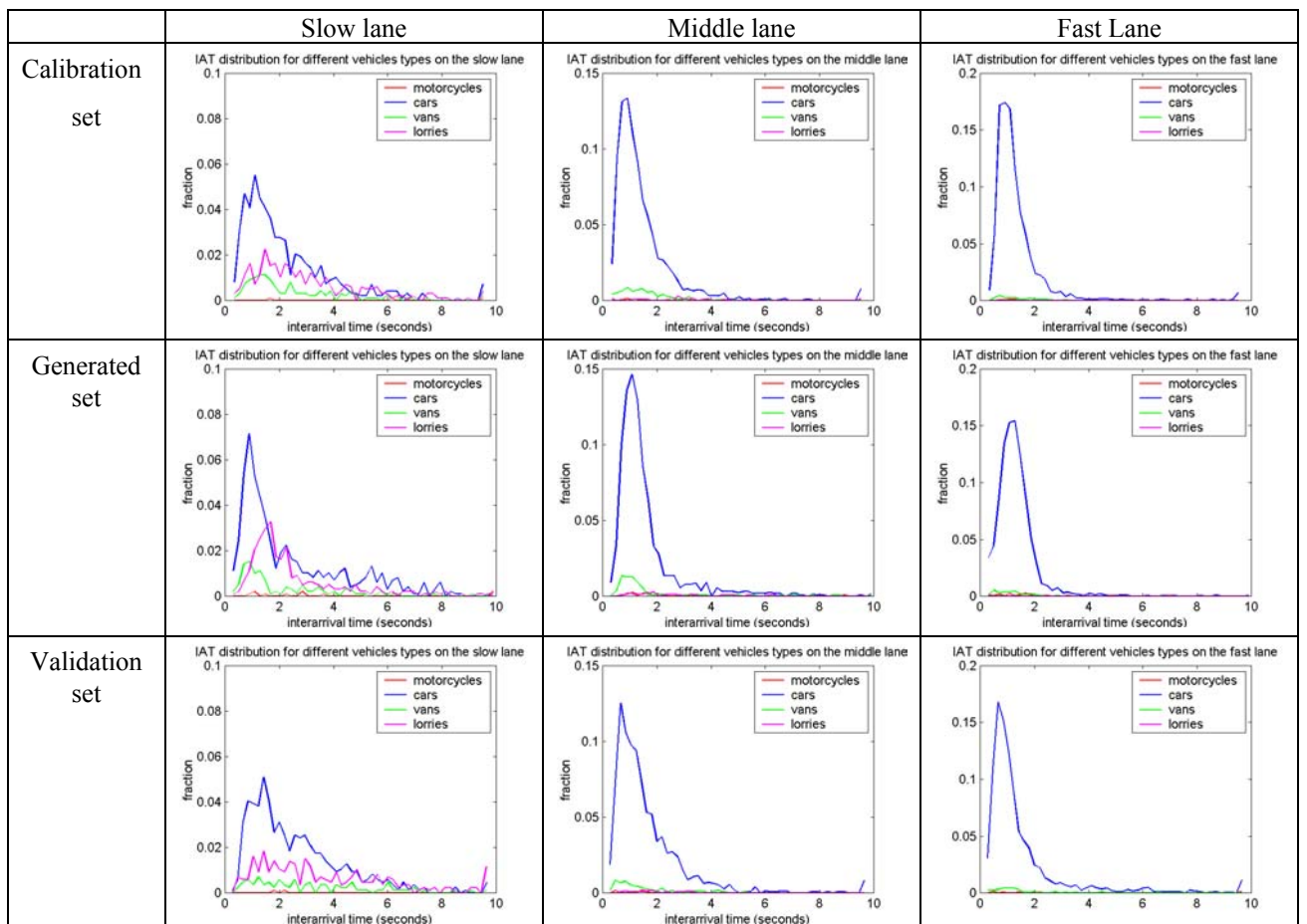
Figure 5: IAT-distributions both measured and generated. Measurements are from the A2 3-lane motorway between Woerden and Utrecht
