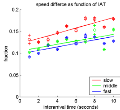
Figure 6: The speed difference ( |\Delta V|/V ) between a vehicle and its predecessor.
