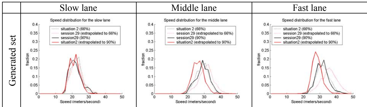
Figure 8: The speed distributions, generated for two volumes I/C.
