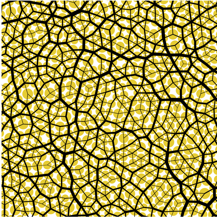
forces in a granular heap
