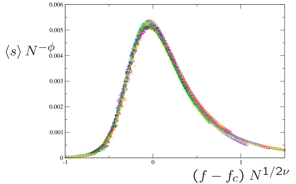
scaling function for force lines
