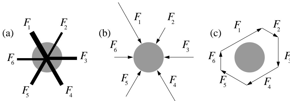
Balanced forces on single grain
