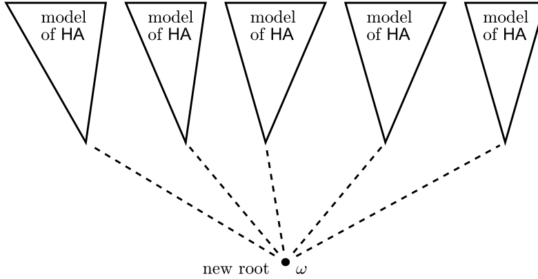
FIGURE 1. Scheme of lemma 5.1: A new model of HA is constructed by equipping a set of models of HA with a new root, and attaching the standard model \omega to it.
