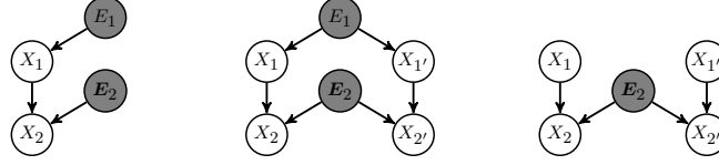
Fig 7: The augmented graph of the SCM \mathcal{M}_\rho (left), its twin SCM \mathcal{M}_\rho^{\text{twin}} (center) and the intervened twin SCM (\mathcal{M}_\rho^{\text{twin}})_{\text{do}(\{1',1\},(1,0))} (right) of Example D.7.
