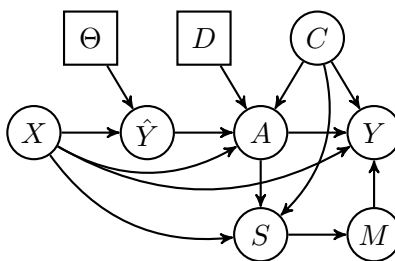
Figure 5: A causal graph with selection variable S .
