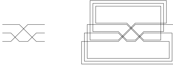
Figure 34: The construction of the pseudocircle arrangement \mathcal{C} (right) from a simple pseudoline arrangement \mathcal{L} (left).
