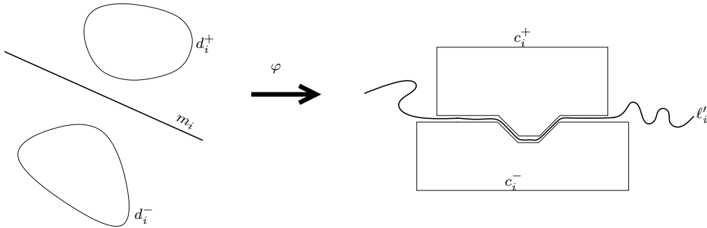
Figure 36: A line m_i separating d_i^- and d_i^+ (left) and their images under \varphi (right).
