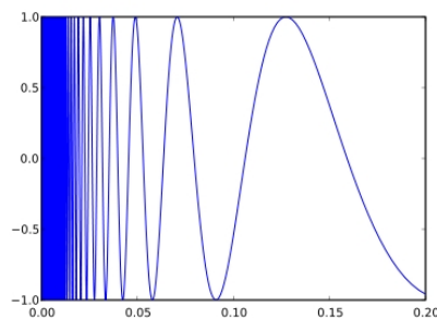
Figuur 12: Topologist's sine curve.
