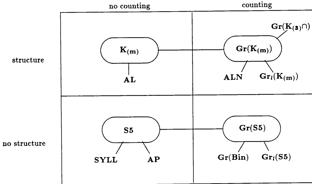
Figure 1: A plethora of calculi.
