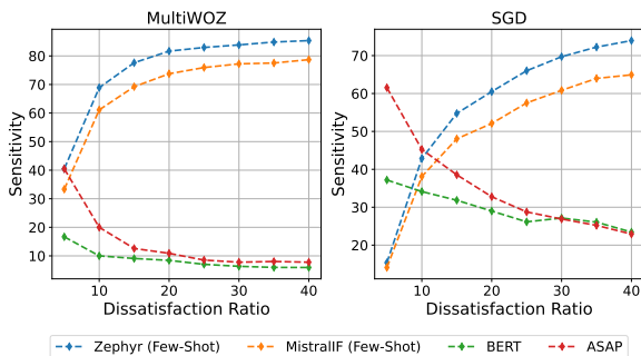
Figure 5: Sensitivity of models in identification of user dissatisfaction on various proportion of Dissatisfaction test samples.
