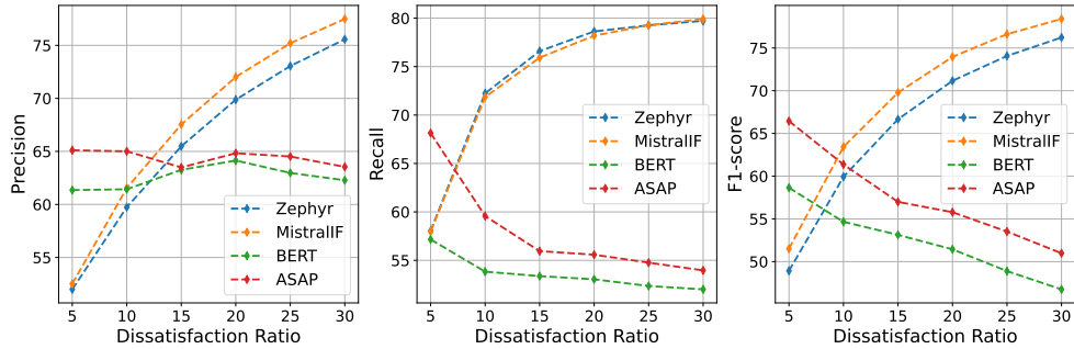
Figure 4: Performance of USE models with a varying degree of imbalance in the test set for the MultiWOZ benchmark. The dissatisfaction ratio is the proportion of samples with dissatisfaction labels in the test collection.
