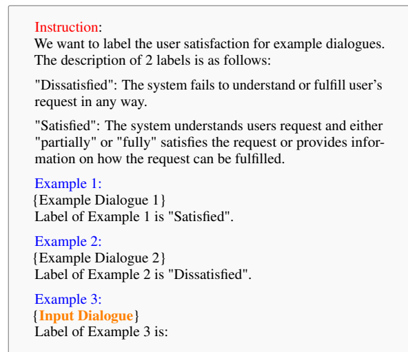
Figure 3: The input used as the prompt for LLMs in order to predict the user satisfaction label.
