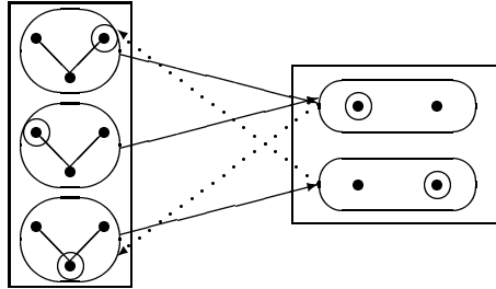
Fibering a tree and an equivalence relation
