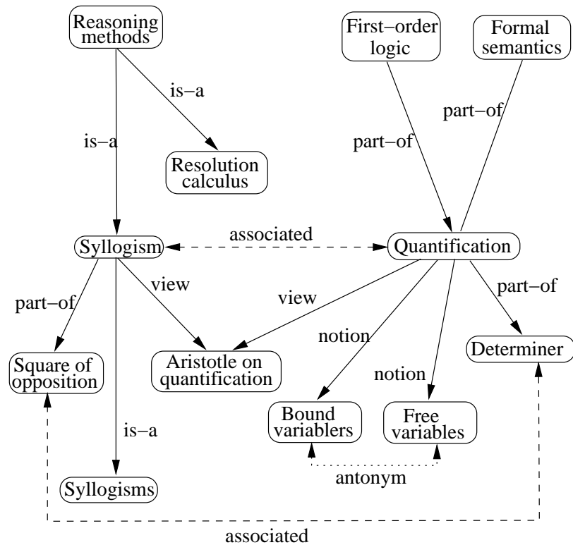
Figure 1: A graphical representation of a fragment of the LoLa concept hierarchy.
