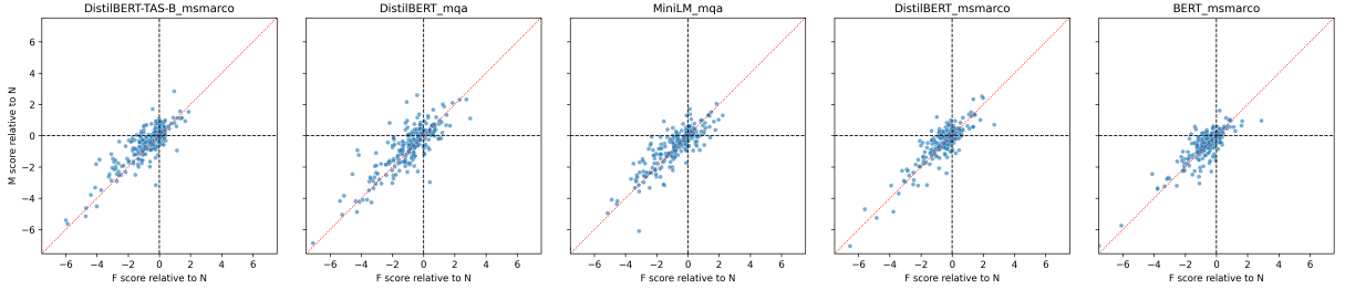
Figure 5: Per-document score differences \Delta_{f-n} (x-axis) and \Delta_{m-n} (y-axis) for all models. Points above the red y = x diagonal indicate that D_m scores higher than D_f relative to D_n .
