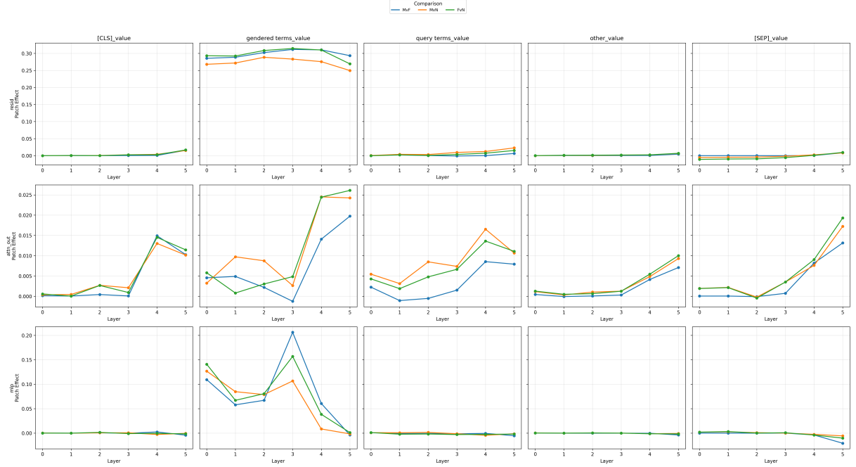
Figure 9: Activation patching results for DistilBERT ms-marco .
