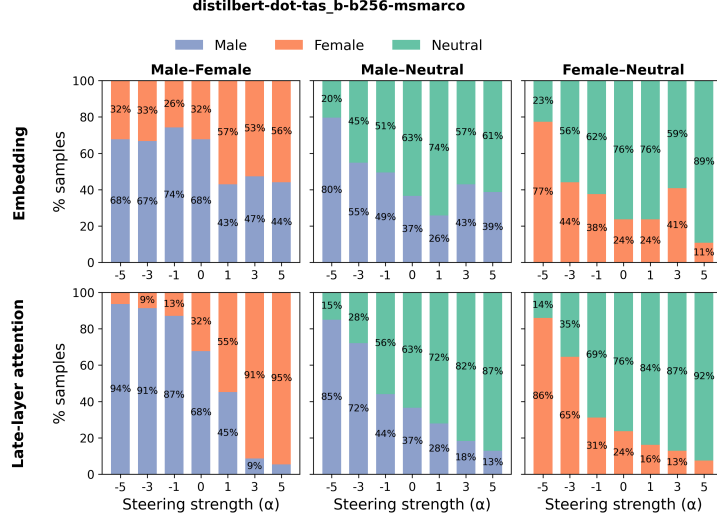
Figure 16: Steering effects on the embeddings (top) compared to attention (bottom) for TAS-B ms-marco , with \alpha \in [-5, 5] in increments of 2 compared to the baseline ( \alpha = 0 ). Percentages refer to the proportion of documents for the given gender that score higher than the other.
