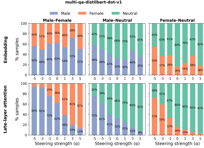
Figure 17: Steering effects on the embeddings (top) compared to attention (bottom) for DistilBERT multi-qa .
