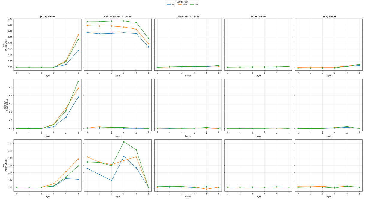
Figure 8: Activation patching results for MiniLM multi-qa .
