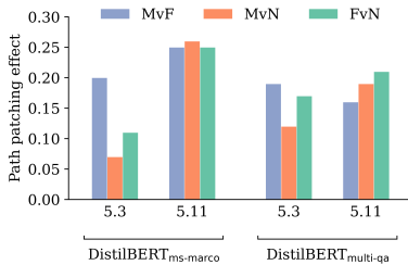
Figure 2: Path patching results to the final residual stream. Full upstream results in Appendix D.2.
