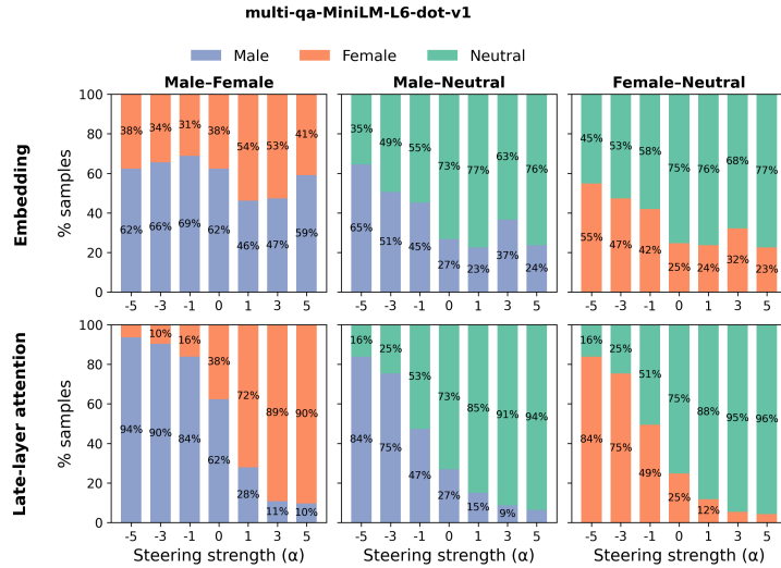
Figure 18: Steering effects on the embeddings (top) compared to attention (bottom) for Mini-LM multi-qa .
