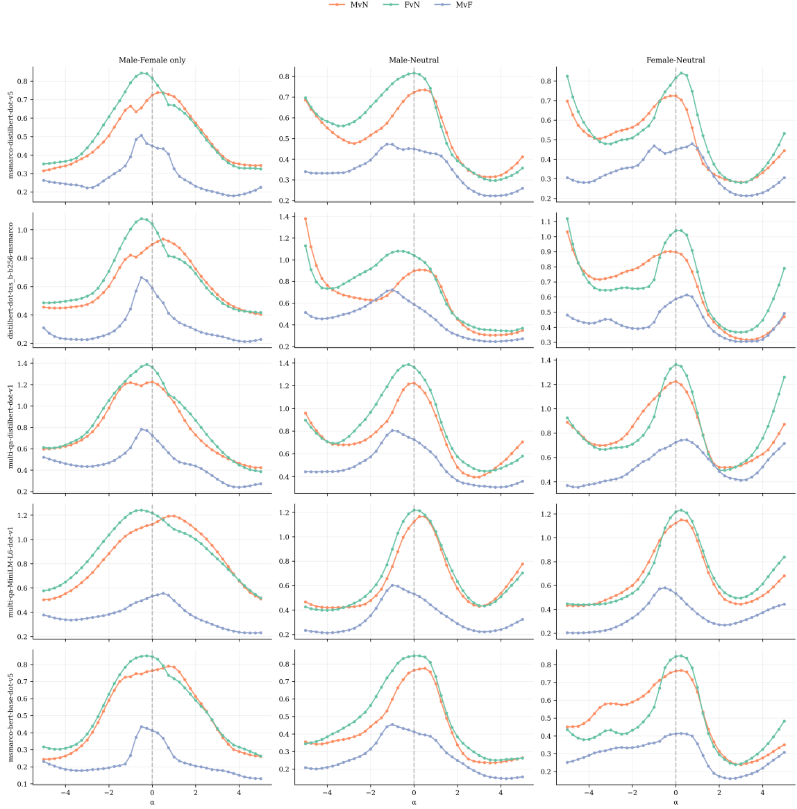
Figure 14: Embedding steering results for all five models for all comparison directions, with \alpha \in [-5, 5] in 0.25 increments.
