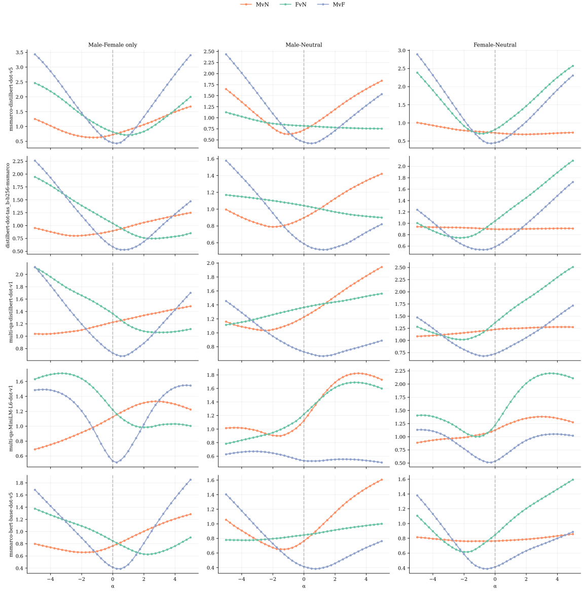
Figure 15: Head steering results for all five models for all comparison directions, with \alpha \in [-5, 5] in 0.25 increments.
