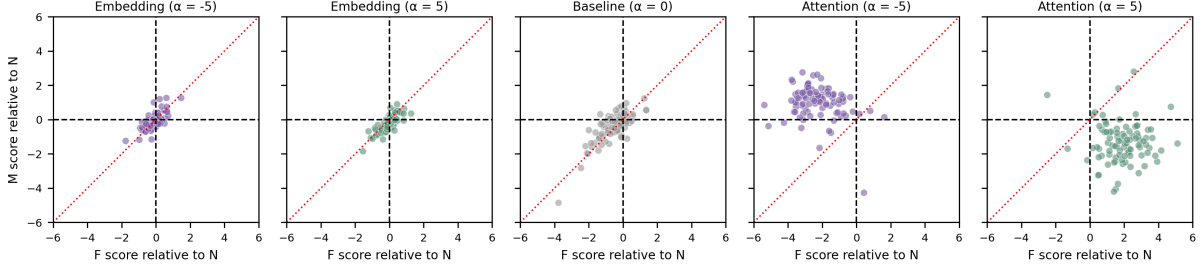
Figure 4: DistilBERT ms-marco steered along the MvF direction at the embedding (left) and late-layer attention (right) levels, compared to the baseline (center).
