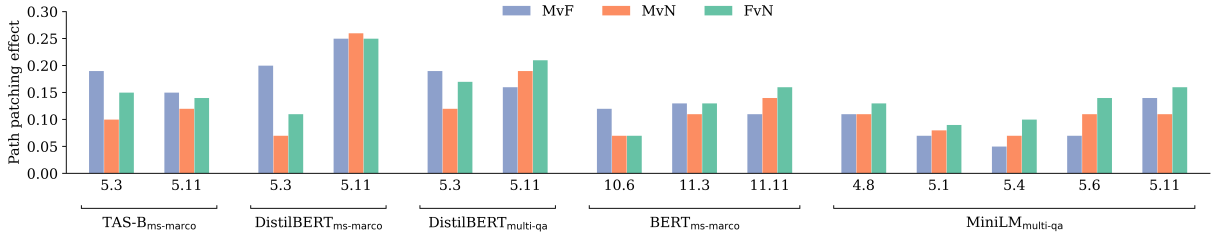
Figure 11: Path patching to the final residual stream for all models.
