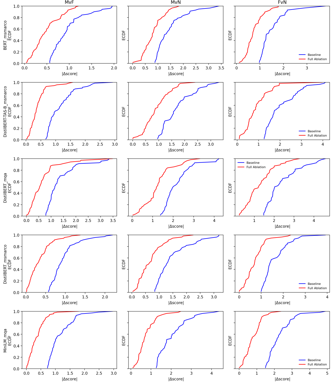
Figure 13: Mean ablation results filtering out documents where the neutral variant’s gendered term appears in the query; top 30 percent of score differences.
