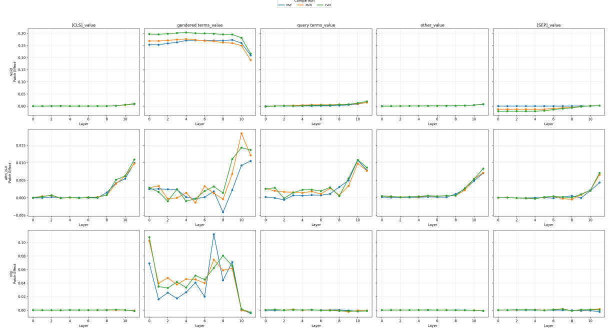
Figure 10: Activation patching results for BERT ms-marco .
