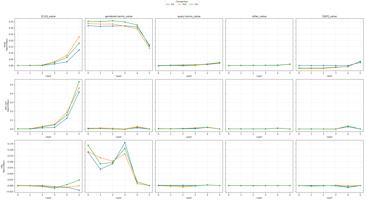
Figure 6: Activation patching results for TAS-B ms-marco .
