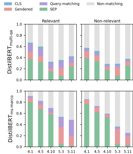
Figure 3: Attention from the CLS ( \text{DistilBERT}_{\text{multi-qa}} , top) and gendered tokens ( \text{DistilBERT}_{\text{ms-marco}} , bottom) to other tokens at heads identified via path patching.
