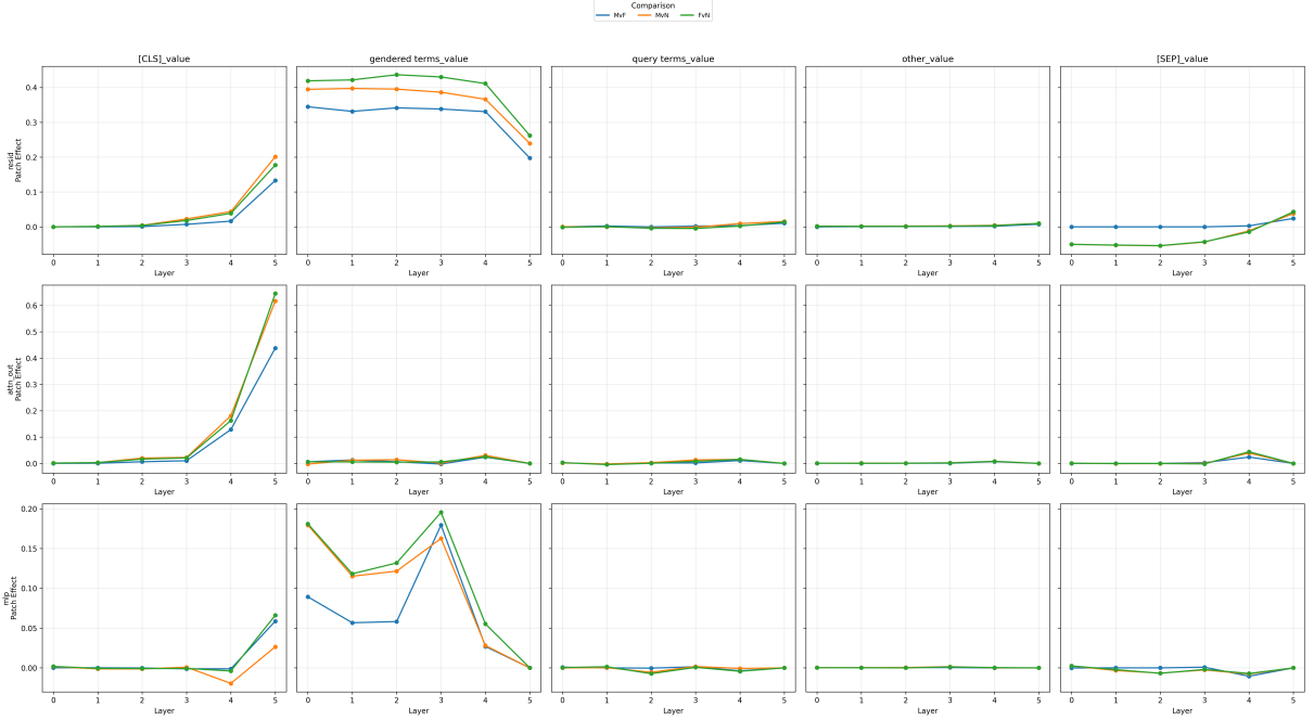
Figure 7: Activation patching results for DistilBERT multi-qa .
