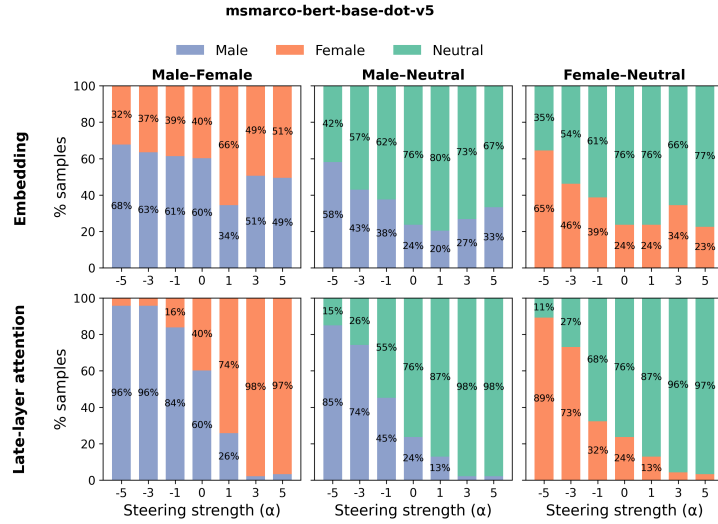
Figure 20: Steering effects on the embeddings (top) compared to attention (bottom) for BERT ms-marco .
