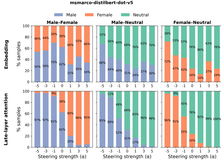
Figure 19: Steering effects on the embeddings (top) compared to attention (bottom) for DistilBERT ms-marco .
