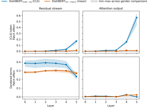
Figure 1: Activation patching effects averaged across the three gender comparisons.
