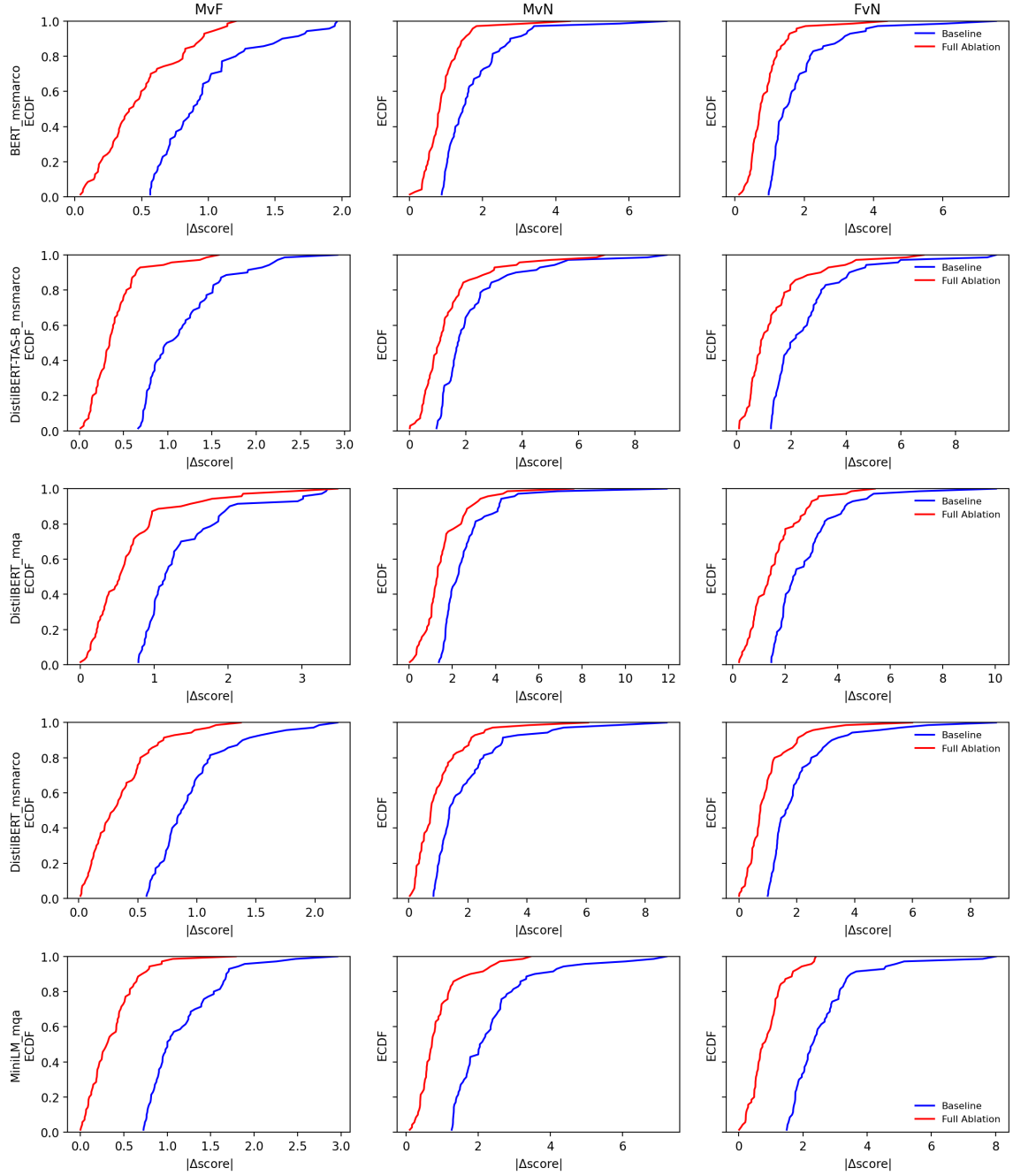
Figure 12: Mean ablating identified heads from path patching; top 30 percent of score differences.
