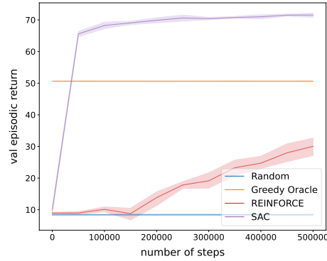
(c) Return (↑) on SingleItem-BoredInf
