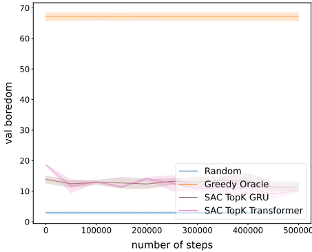
(c) SlateTopK-Uncertain, high uncertainty
