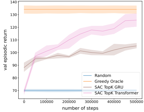
(b) SlateTopK-Uncertain, medium uncertainty
