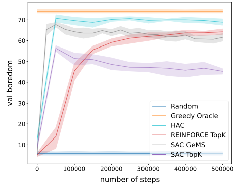
(b) Boredom (↓) on SlateTopK-Bored (Ideal)
