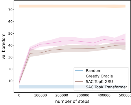
(a) SlateTopK-PartialObs, low uncertainty
