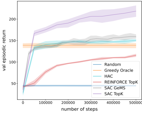
(a) Return (↑) on SlateTopK-Bored (Ideal)
