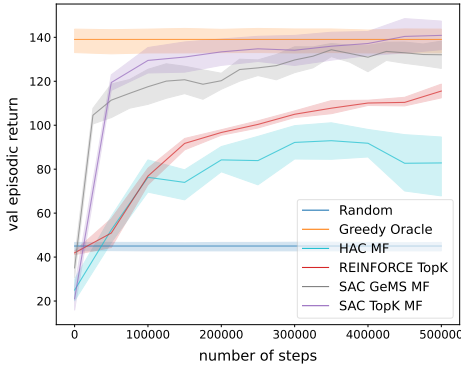
(c) Return (↑) on SlateTopK-Bored (MF)
