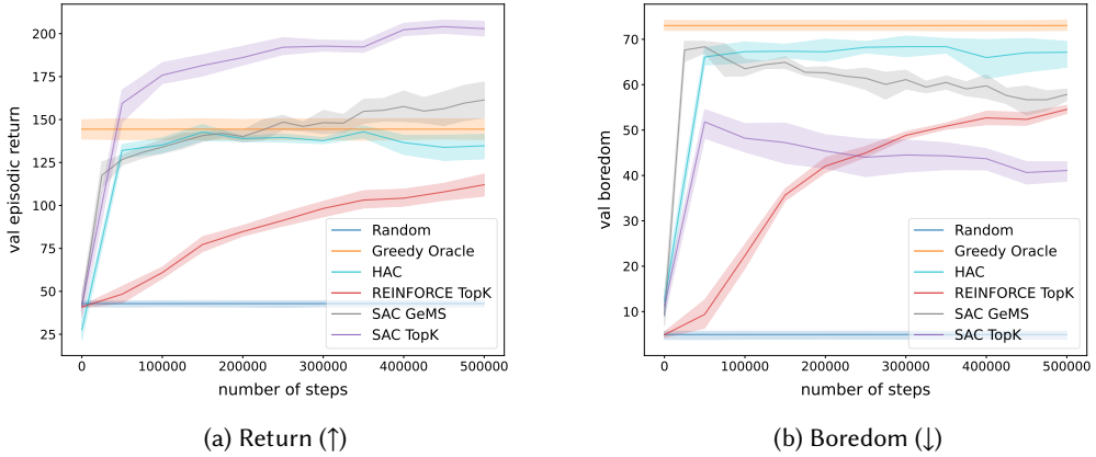
Fig. 4. Results on the SlateTopK-BoredInf environment. The colored envelope surrounding lines indicates the 95% confidence interval around the mean computed from 5 seeded runs.
