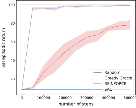
(a) Return (↑) on SingleItem-Static
