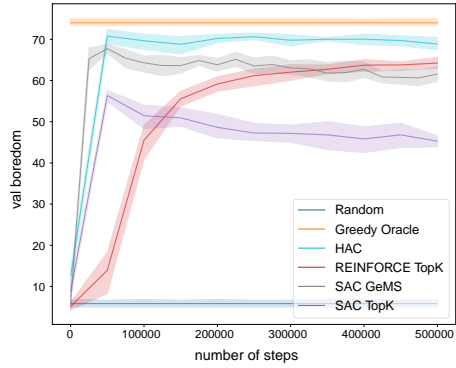
(b) Boredom ( \downarrow ) on SlateTopK-Bored (Ideal)
