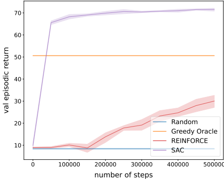
(c) Return (↑) on SingleItem-BoredInf
