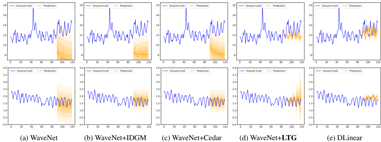
Figure 7: Forecasting results for test domain samples from the Web-traffic dataset, using DLinear and WaveNet with various generalization methods. Each row represents a different sequence example.
