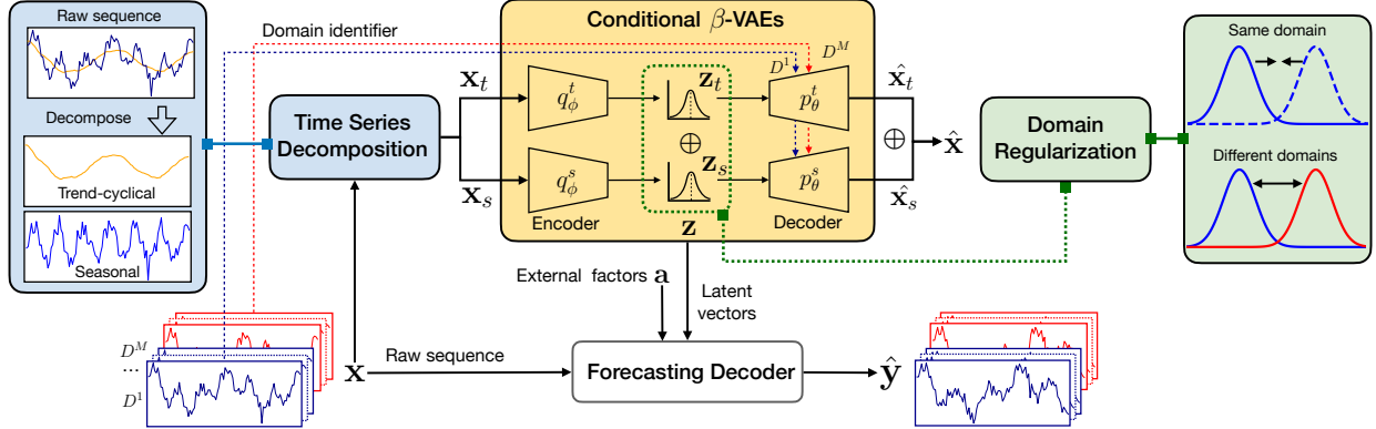
Figure 1: The proposed framework, LTG , consists of three components: (1) Time Series Decomposition, which decomposes a raw time sequence into trend-cyclical and seasonal components for more effective modeling of distinct temporal patterns. (2) Latent Factor Learning with Conditional \beta -VAE, which learns latent representations that capture temporal dependencies across different domains and ideally achieves disentangled latent factors for each dimension. (3) Domain Regularization, which regularizes domain-specific and shared latent features to enhance the disentangling of latent factors. The forecasting decoder is a flexible model that integrates the raw sequence, any external factors, and the latent vectors learned by the Conditional \beta -VAE to generate time series forecasts.
