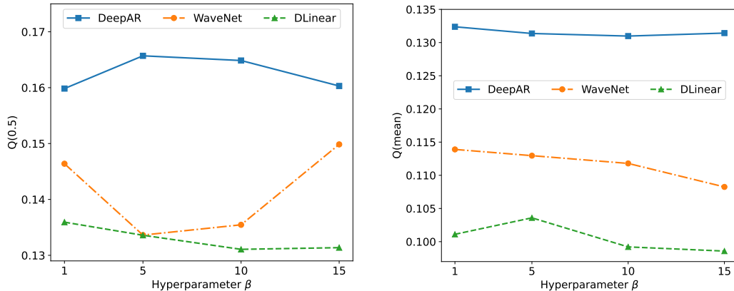
Figure 5: Forecasting results of Q(0.5) and Q(\text{mean}) on the Web-traffic dataset with varying values of \beta .
