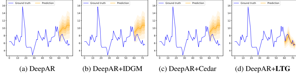
Figure 8: Forecasting results for a test domain sample from the Stock-volume dataset, using DeepAR with various generalization methods.
