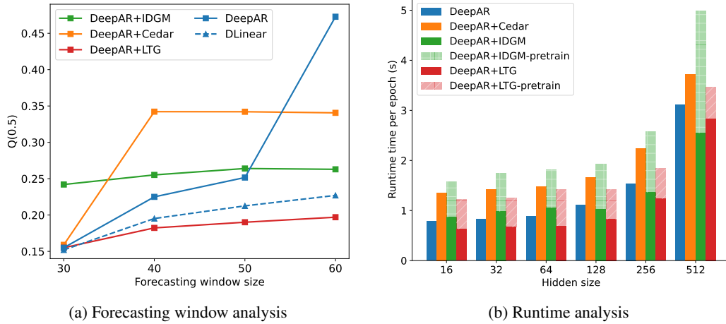
Figure 4: Forecasting window sensitivity and runtime analysis on the Web-traffic dataset using DeepAR as the base model.
