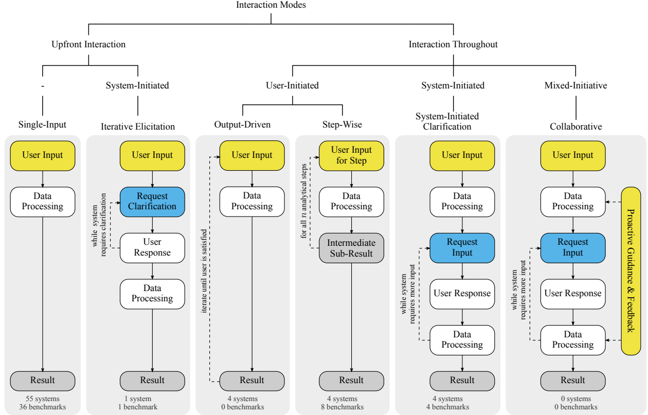
Figure 8: Interaction modes organized by interaction timing, whether input occurs only upfront or continues during execution, and interaction initiative. Counts state how many of the 58 reviewed systems and 42 benchmarks support the respective mode. Counts are not mutually exclusive; 7 systems and 7 benchmarks support more than one mode.
