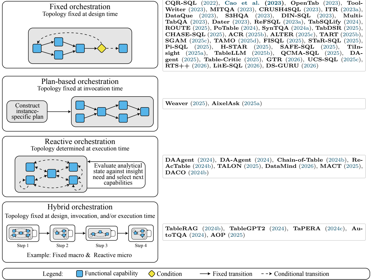
Figure 7: Overview of orchestration strategies alongside works that employ the respective strategies. The schematic in each row depicts the corresponding control flow.
