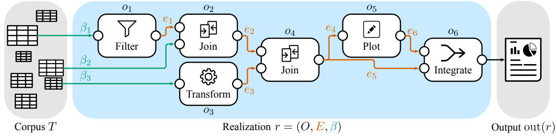
Figure 3: Example of an abstracted realization r = (O, E, \beta) . Nodes are fully parameterized operations O , edges E denote dataflow, and the binding \beta anchors source operations to corpus tables. The graph converges to a single sink operation producing the output.
