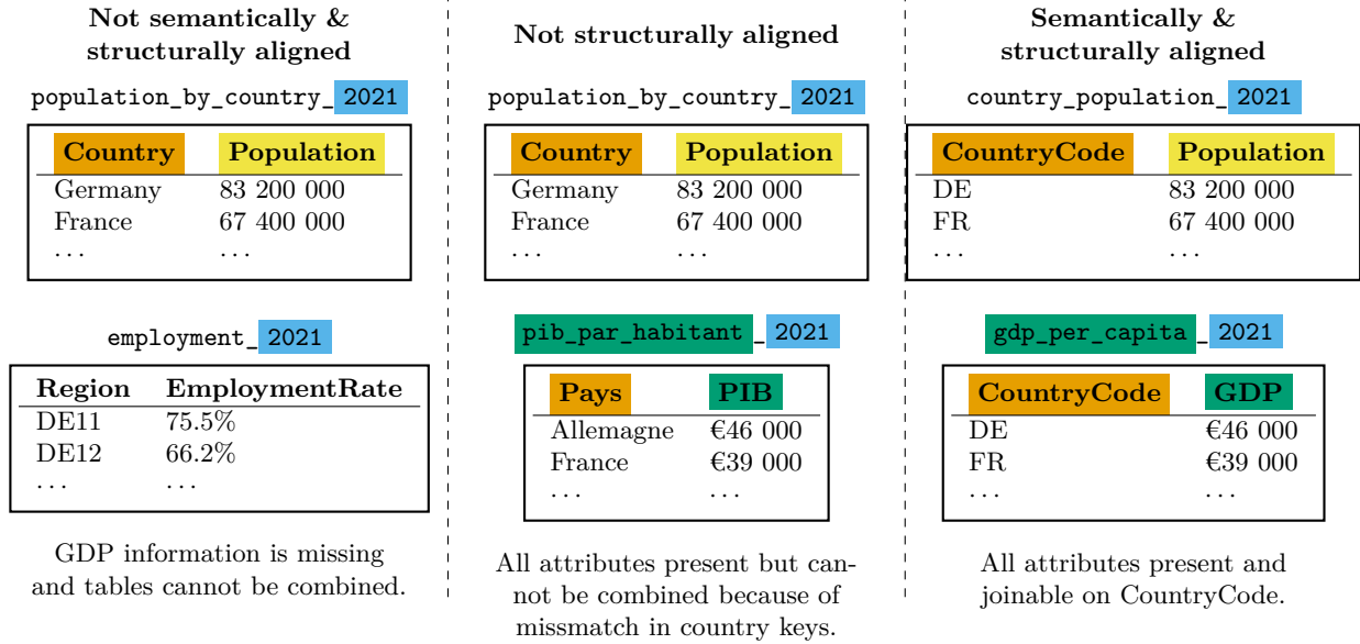
Figure 4: Example of semantic and structural alignment. A candidate set is semantically aligned when its tables jointly cover the required concepts and structurally aligned when they are combinable, here via a join on CountryCode. Both must hold for sufficiency.
