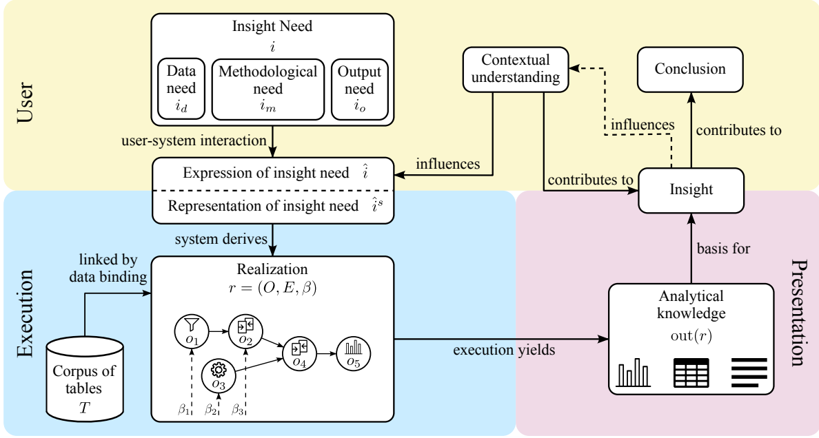
Figure 2: Relationships and dependencies among core concepts of OpenTI. A user holds an insight need i , consisting of a data need i_d , methodological need i_m , and output need i_o , and expresses it as \hat{i} . A system maps \hat{i} to a realization r = (O, E, \beta) , a graph of operations O connected by dataflow edges E with a binding \beta that links operations to tables from the corpus T . Executing r yields analytical knowledge as output \text{out}(r) , which is the basis for an insight.
