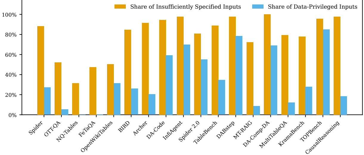
Figure 10: Share of inputs that are insufficiently specified (i.e., admitting multiple interpretations) and that exhibit data privileges (i.e., leakage of privileged information from the data into the input) across benchmarks.
