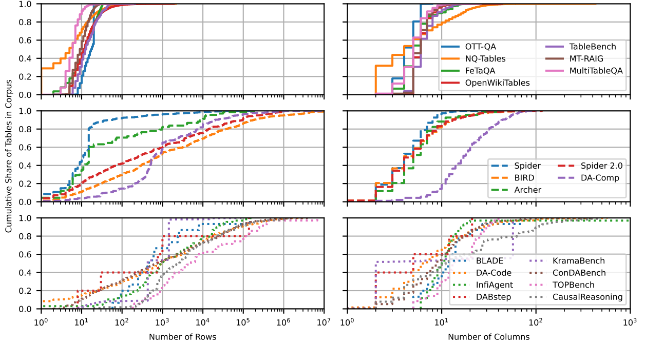
Figure 9: Empirical cumulative distributions of per-table row and column counts for the corpora in Table 2. Steep curves at low counts mark corpora of small tables, while flatter curves indicate diversity in row and column counts.
