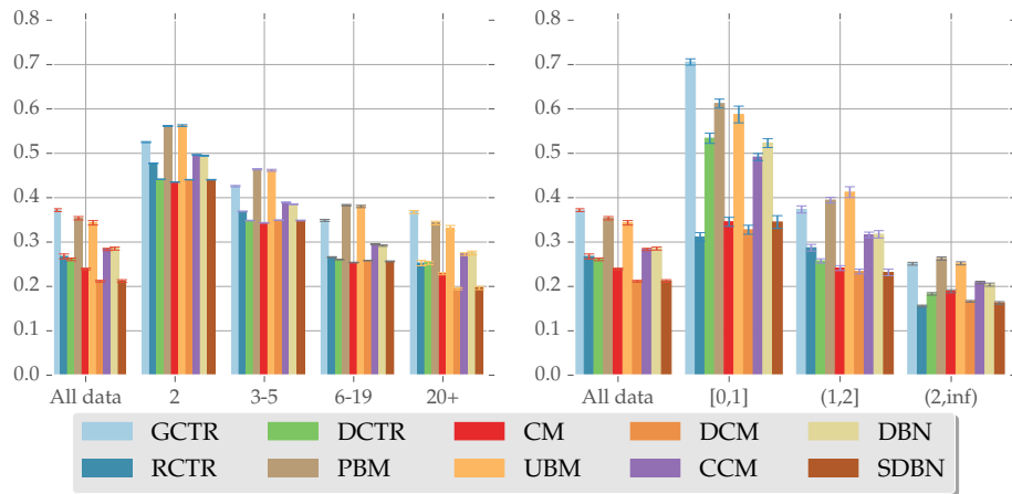
Fig. 3: Click-through rate prediction RMSE of click models, grouped by query frequency (left) and click entropy (right).
