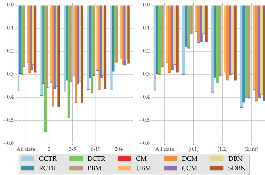
Fig. 1: Log-likelihood of click models, grouped by query frequency (left) and click entropy (right).
