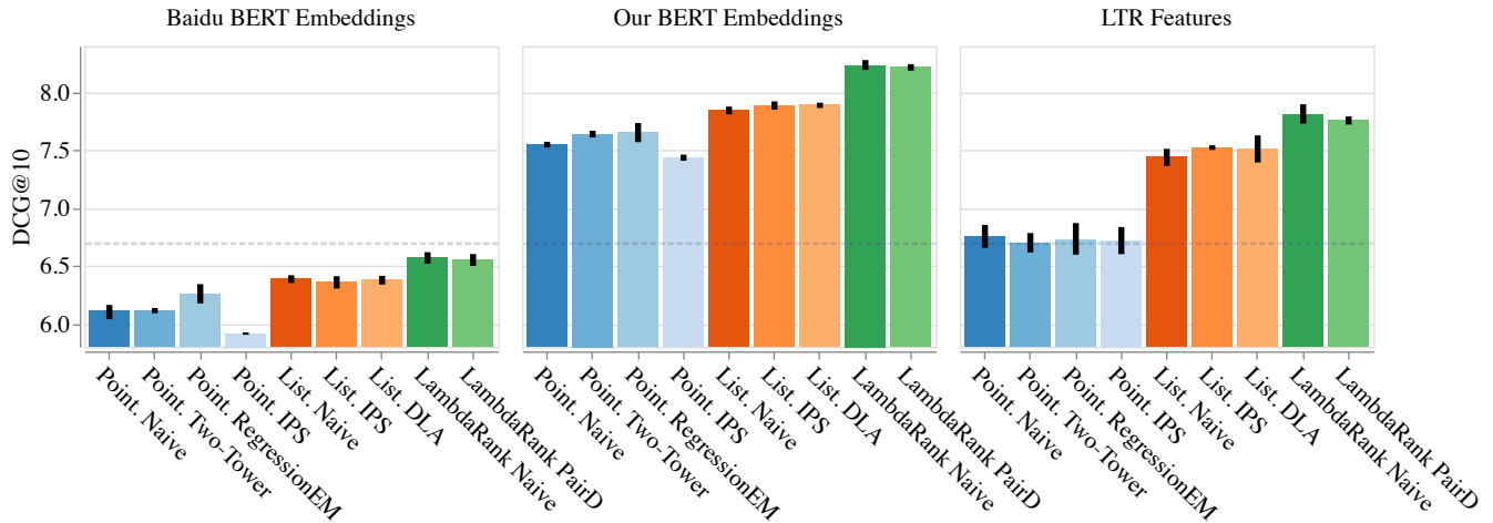
Figure 3: Comparing ULTR method on pre-trained BERT embeddings and LTR features. We display the average ranking performance measured in DCG@10 over five independent runs and plot a bootstrapped 95% confidence interval. The grey dotted line indicates the performance of a random ranker.
