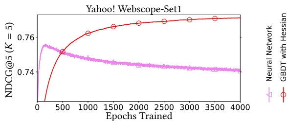
Figure 3: Convergence analysis on the Yahoo! dataset.
