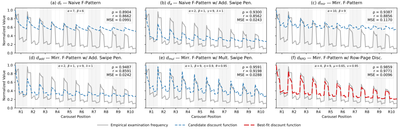
Figure 2: Fitted parameters and test-set performance ( \rho , r , MSE) of each discount function are reported. Both the empirical examination frequencies and the computed discounts are max-normalized to [0, 1] before plotting and MSE evaluation, so the comparison reflects how well each formulation captures the relative decay of user attention rather than its absolute magnitude.
