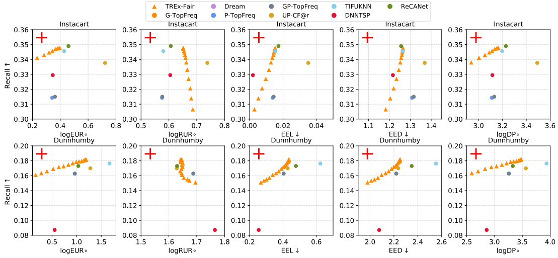
Figure 5: Performance of TREx_{Fairness} at different v values, compared with different NBR methods in terms of different fairness metrics. The red + marker indicates the direction with both high accuracy and fairness.
