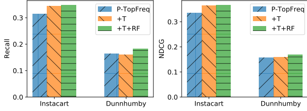
Figure 2: Performance of TREx-Rep when we add a time-decay factor \beta (+T), add both \beta and item-specific repetition feature RepI(i) (+T+RF).
