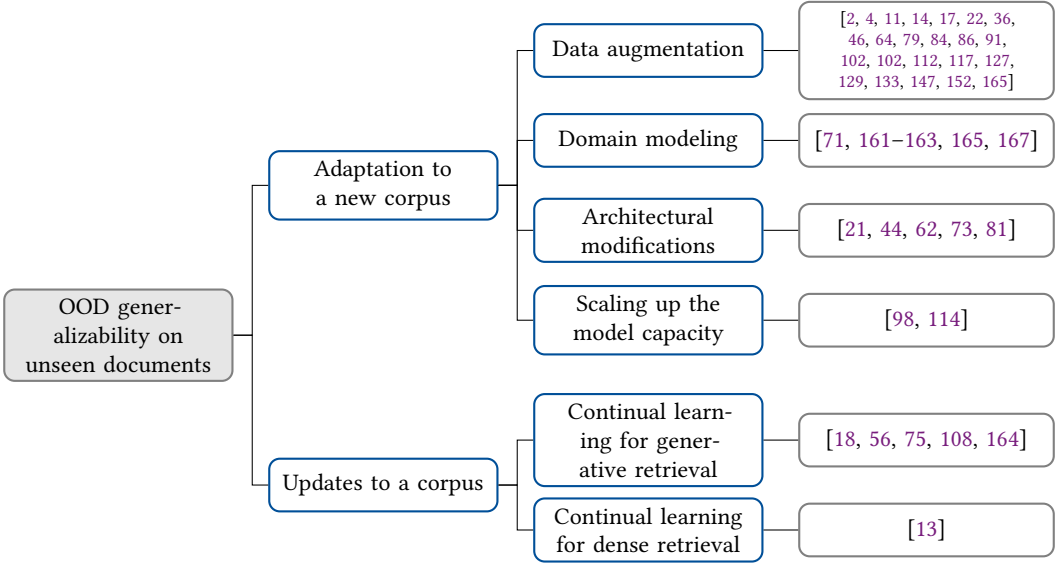
Fig. 10. Classification of OOD generalizability on unseen documents.
