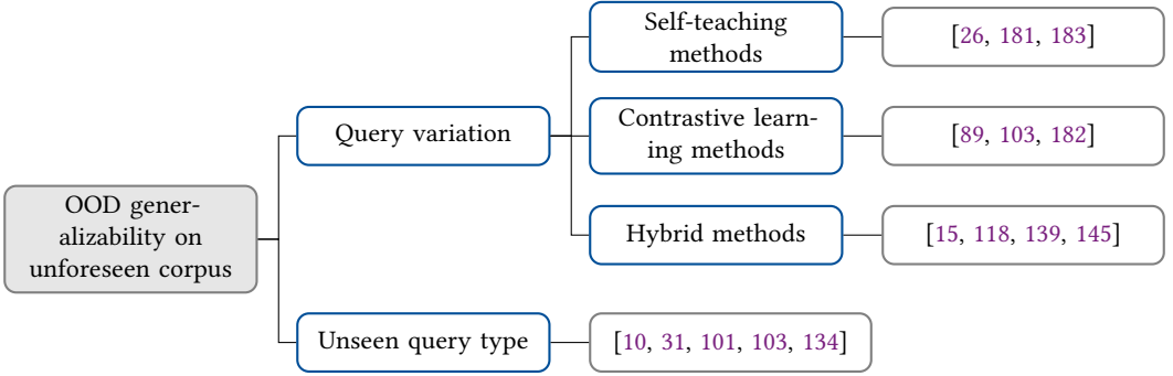
Fig. 11. Classification of OOD generalizability on unseen queries.
