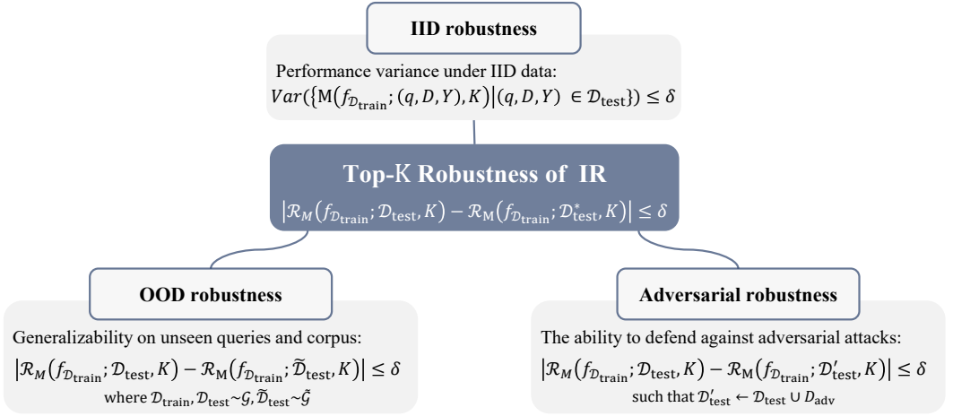
Fig. 4. A taxonomy of robustness in IR. In this survey, we pay special attention to adversarial robustness and OOD robustness.
