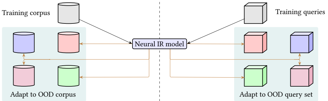
Fig. 9. OOD generalizability on unseen documents vs. queries in neural IR.
