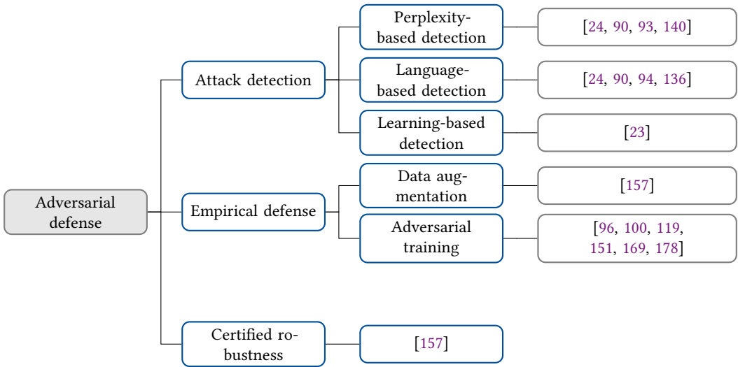
Fig. 8. Classification of adversarial defenses in neural IR.
