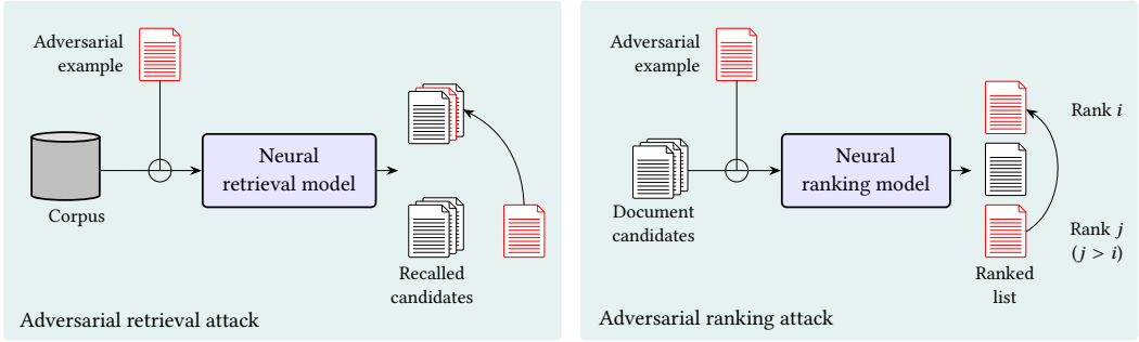
Fig. 6. Adversarial retrieval attacks vs. adversarial ranking attacks.
