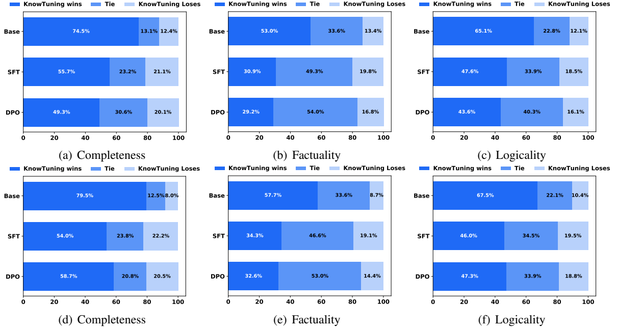
Figure 3: Results on unseen QA datasets evaluated by GPT-4, including completeness, factuality, and logicity. The backbone model of (a), (b) and (c) is Llama2-7b-base. The backbone model of (d), (e) and (f) is Llama2-13b-base.
