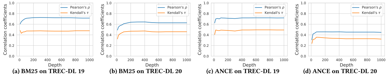
Figure 2: Relationship between the QPP effectiveness of predicting nDCG@10 and the judging depth for a ranked list.
