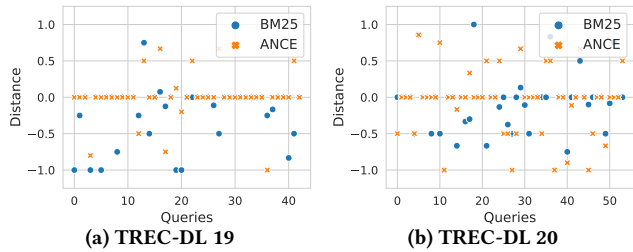
Figure 3: QPP errors in predicting the performance of BM25 and ANCE in terms of RR@10 on TREC-DL 19, 20. The distance is defined as “predicted RR@10 minus actual RR@10.”
