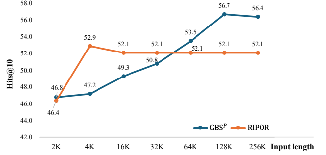
Figure 3: The performance, in terms of Hits@10, of GBS^P and RIPOR with different input lengths on the BBS 40K dataset.
