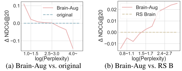
Figure 2: Relationship between document ranking performance and perplexity of ground-truth query continuation in Pereira’s dataset. “RS B” indicates the ablation of Brain-Aug that randomizes brain inputs. \Delta NDCG@20 indicates performance gains of Brain-Aug.
