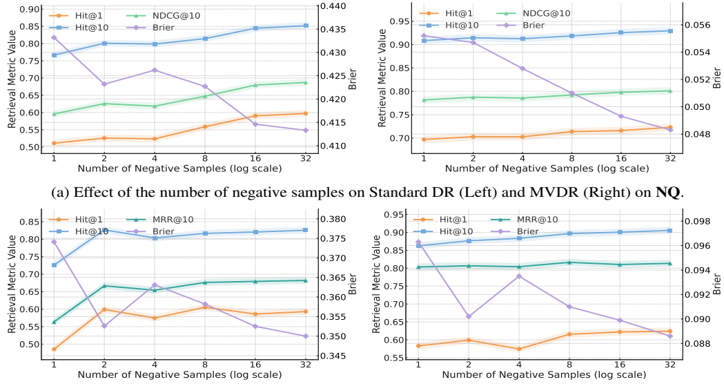
(a) Effect of the number of negative samples on Standard DR (Left) and MVDR (Right) on NQ .
