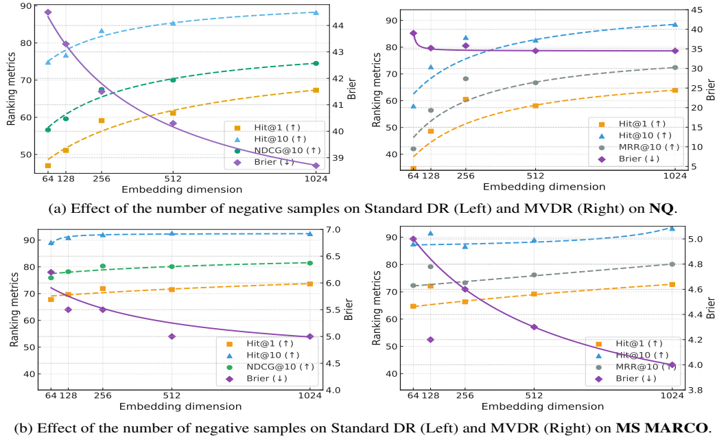
Figure 2: DR’s retrieval performance improves as the embedding dimension increases.
