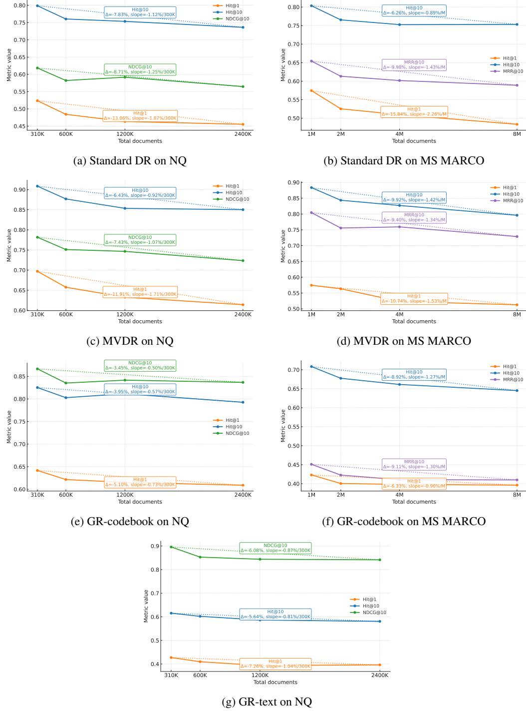
Figure 4: Extended results of corpus scaling.
