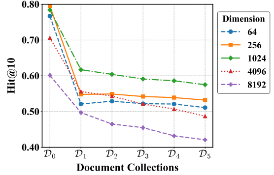
Figure 3: Hit@10 performance of different decoding dimension of Ultron-PQ on NQ dataset
