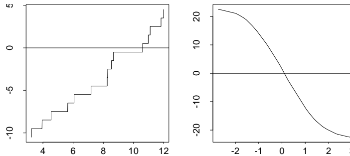
Figure 4.1. The functions \theta \rightarrow \Psi_n(\theta) for the 80%-quantile and the Huber estimator for samples of size 15 from the gamma(8,1) and standard normal distribution, respectively.
