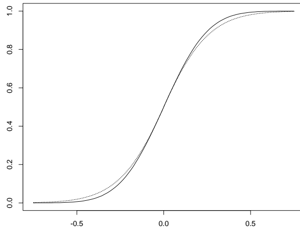
Figure 4.2. The distribution function of the sample median (dotted curve) and its normal approximation for a sample of size 25 from the Laplace distribution.
