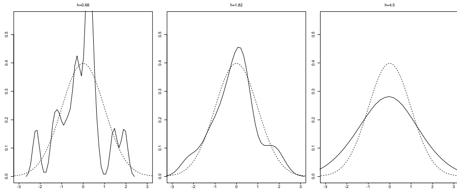
Figure 5.3. Kernel estimates for the density of a sample of size 15 from the standard normal density for three different bandwidths, using a normal kernel. The dotted line gives the true density.
