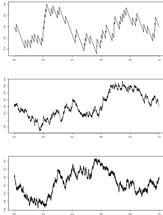
Figure 5.1. Three realizations of the uniform empirical process, of 50, 500 and 5000 observations, respectively.
