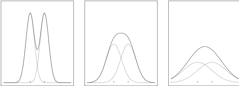
Figure 5.2. The kernel estimator with normal kernel and two observations for three bandwidths: small (left), intermediate (middle) and large (right). The figures shows both the contributions of the two observations separately (dotted lines) and the kernel estimator (solid lines), which is the sum of the two dotted lines.
