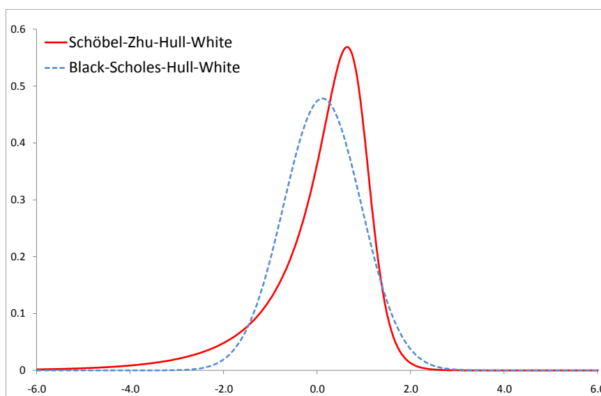
Figure 1: Risk-neutral density of the log-asset price for the SZHW and BSHW model, calibrated to EU market option data.
