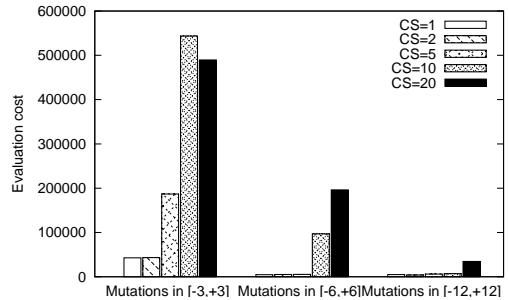
Figure 4: Effects on average evaluation costs when SBA is created by grouping similar behaviors.
