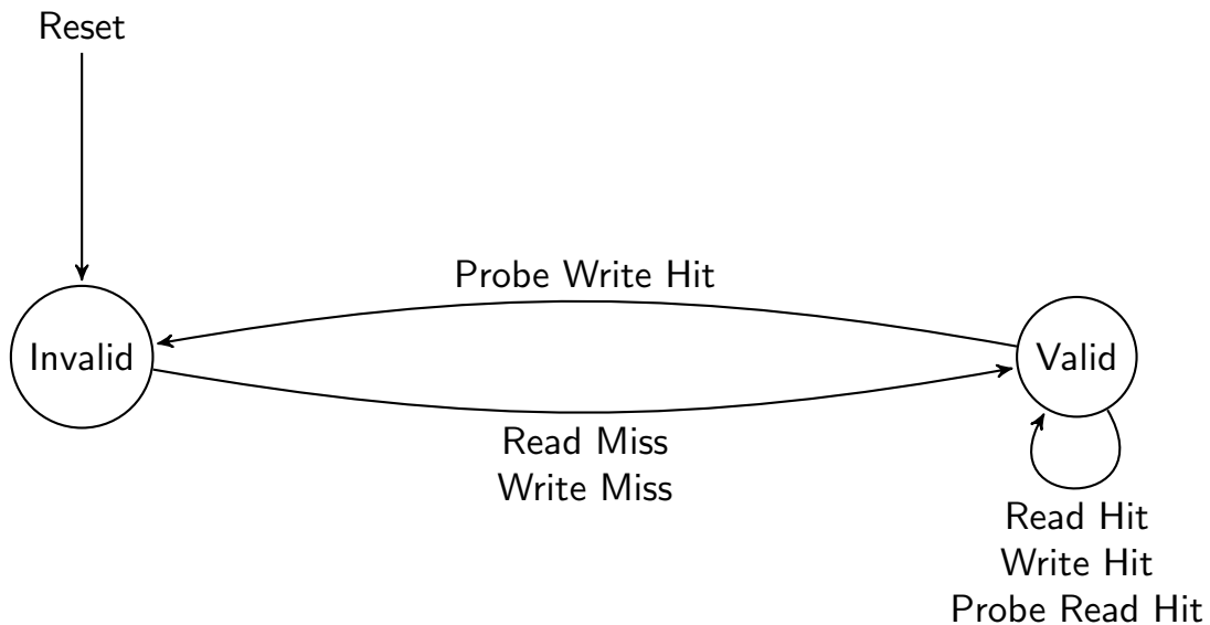
Figure 2: VALID INVALID Cache Line State Transition Diagram.
