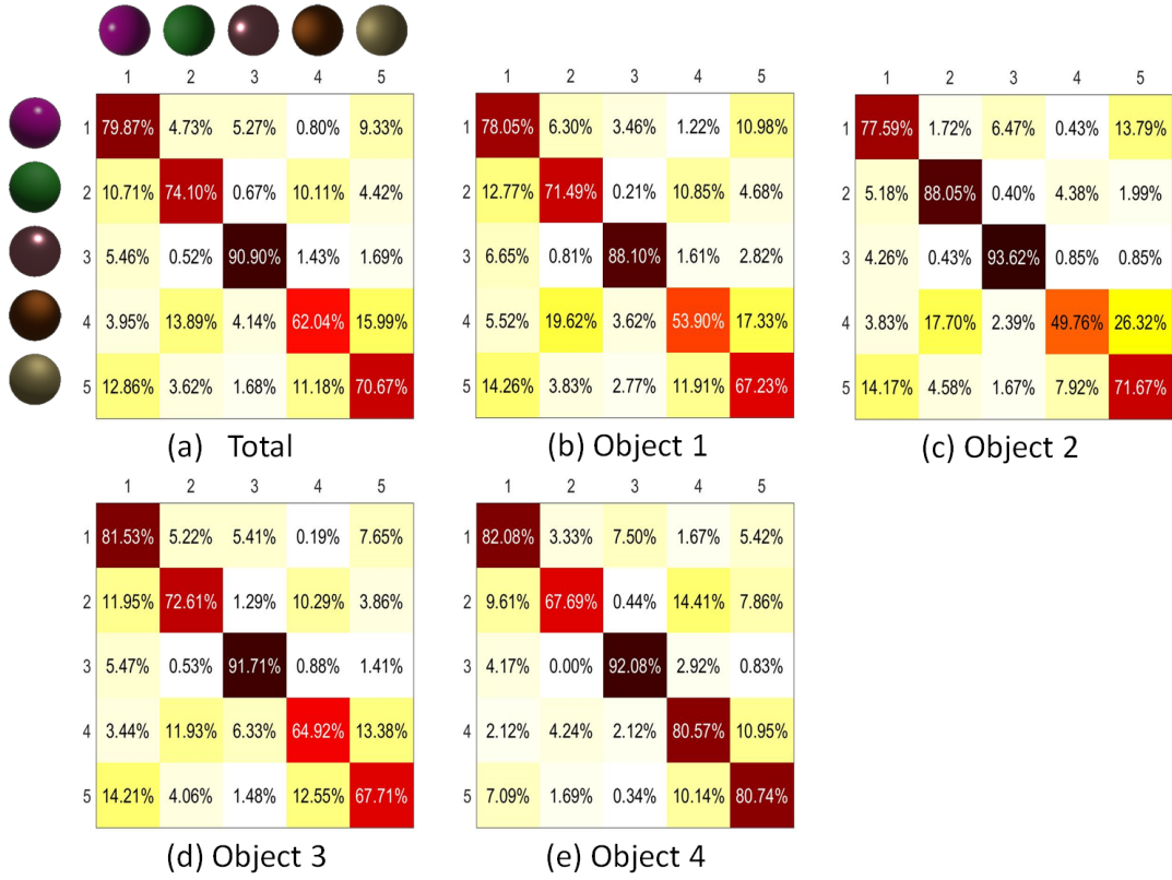
(a) Confusion matrix of the StackNet's results
