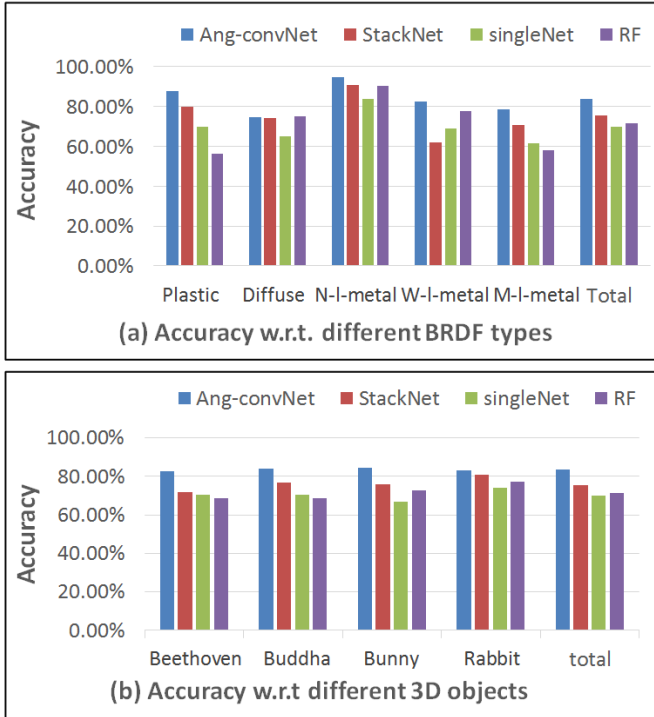
Fig. 7. Comparison of identification accuracy between Ang-ConvNet and StackNet. (a) Accuracy w.r.t. different BRDF types. (b) Accuracy w.r.t. different 3D objects. Five BRDF types include plastic, diffuse, narrow-lobe-metal, wide-lobe-metal, and mid-lobe-metal respectively.
