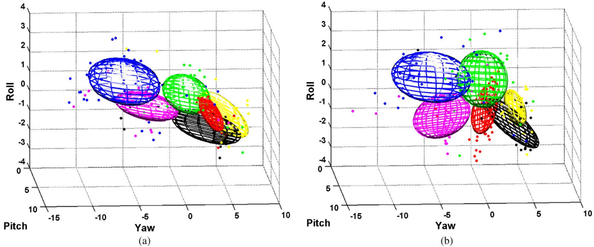
Fig. 7. Distribution of estimated pose values for two video sequences. Each point is a pose value for one object location; ellipsoids are representations for clusters obtained by adapting multivariate Gaussian distributions for each object.
