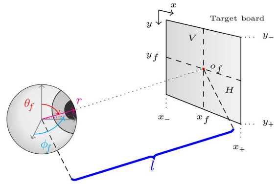
Fig. 4. Orientation of the eyeball model and the attended point.
