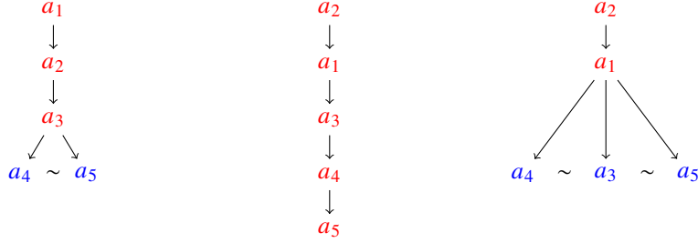
Figure 2: The top alternatives of each single preference are in red. From left to right, these are the sets \{a_1, a_2, a_3\} , \{a_1, \dots, a_5\} , and \{a_1, a_2\} , respectively. The TOPsets(\succsim) of the leftmost preference \succsim are \{\{a_1\}, \{a_1, a_2\}, \{a_1, a_2, a_3\}\} , and similarly for the other preferences. The intersection of these sets is then the set \{a_1, a_2\} , which includes the top alternatives of the whole profile.
