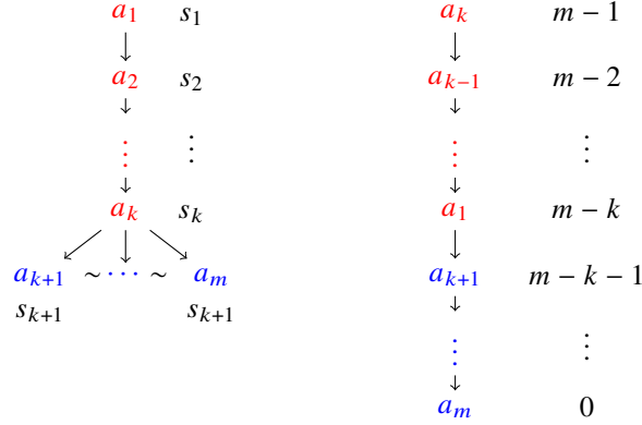
Figure 6: A top-truncated preference \succsim and a linearisation L of it with the order of its top alternatives reversed. We have that s_{\succsim}(a_1) = s_1, \dots, s_{\succsim}(a_k) = s_k, s_{\succsim}(a_{k+1}) = \dots = s_{\succsim}(a_m) = s_{k+1} and s_L(a_k) = m-1, \dots, s_L(a_1) = m-k, s_L(a_{k+1}) = m-k-1, \dots, s_L(a_m) = 0 .
