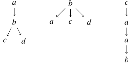
Figure 5: A profile where the pessimistic, the optimistic, and the average Borda rule output different sets of winners: \{b\} , \{a, c\} , and \{a, b\} , respectively.
