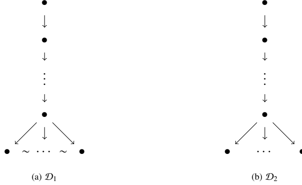
Figure 1: Types of top-truncated preferences in two domains: \mathcal{D}_1 and \mathcal{D}_2 .
