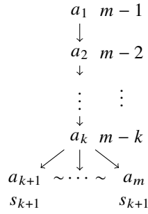
Figure 4: A rule in the Borda class on the domain \mathcal{D}_1 , for s_{k+1} < m - k .
