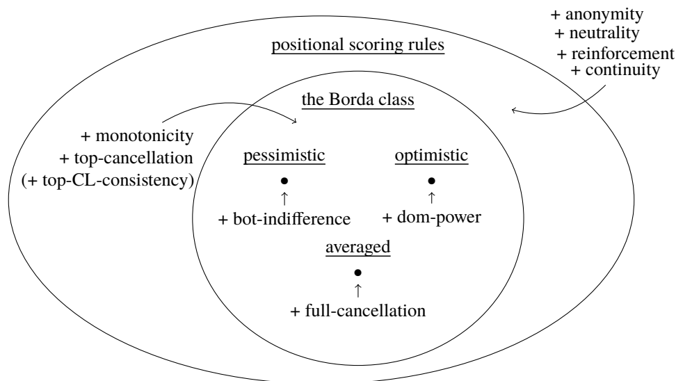
Figure 8: Borda rules for top-truncated preferences and the axioms that characterise them. The axioms next to an arrow indicate those properties that are required in order to obtain a specific class of rules, or a specific rule, within a larger class.
