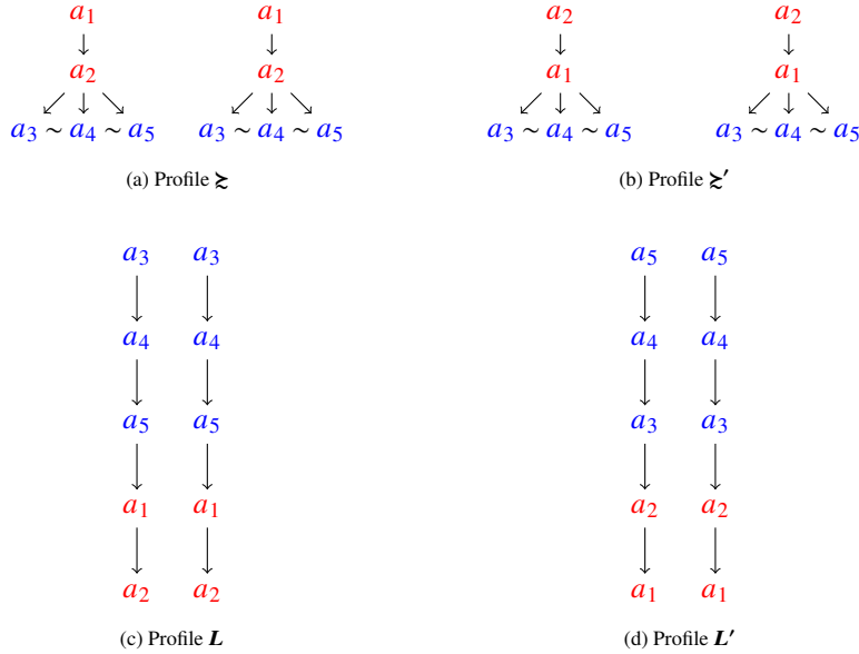
Figure 7: The construction of the profiles appearing in the proof of Theorem 6, for m = 5 and k = 2 .
