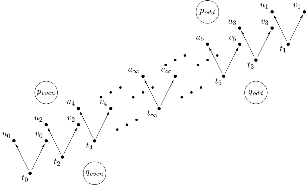
Figure 1: The descriptive model \mathbb{X} of Example 4.6
