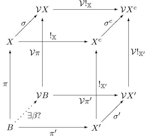
Figure 2: An explicit counterexample to \mathcal{V} preserving weak pullbacks
